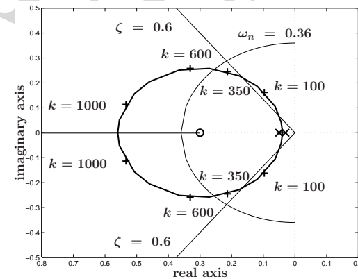
Root Locus and PID Control EEE 151
