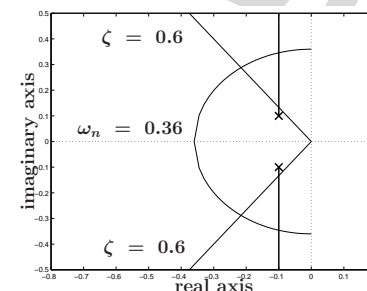
Root Locus and PID Control EEE 151
